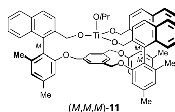
FIGURE 5. Structure of the C 3 -symmetric titanium catalyst ( M,M,M )- 11 .
