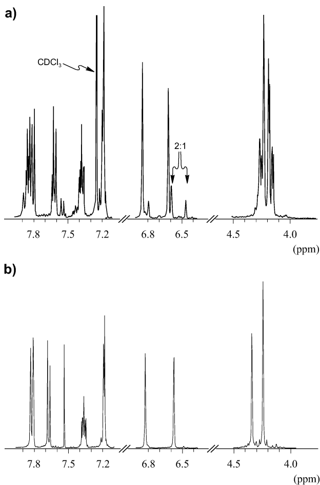
FIGURE 3. Diagnostically decisive part of the ^1\text{H} NMR spectra of ( M,M,M )-3 (a) in \text{CDCl}_3 and (b) in \text{CD}_3\text{OD} .
