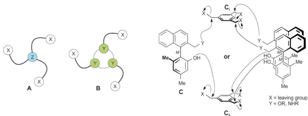
FIGURE 2. Schematic sketches of acyclic and exocyclic C_3 -symmetric systems.
