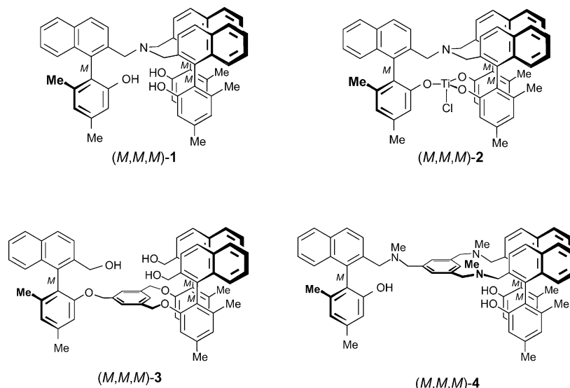
FIGURE 1. The axially chiral tripodal ligand (M,M,M) -1 and its titanium complex (M,M,M) -2, and the concrete target ligands (M,M,M) -3 and (M,M,M) -4.
