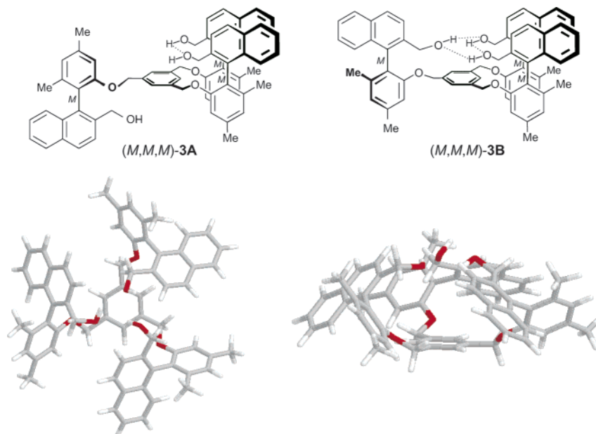
FIGURE 4. Conformers of ( M,M,M )- 3 , ( M,M,M )- 3A , and ( M,M,M )- 3B , and the AM1-calculated minimum structure of ( M,M,M )- 3B .
